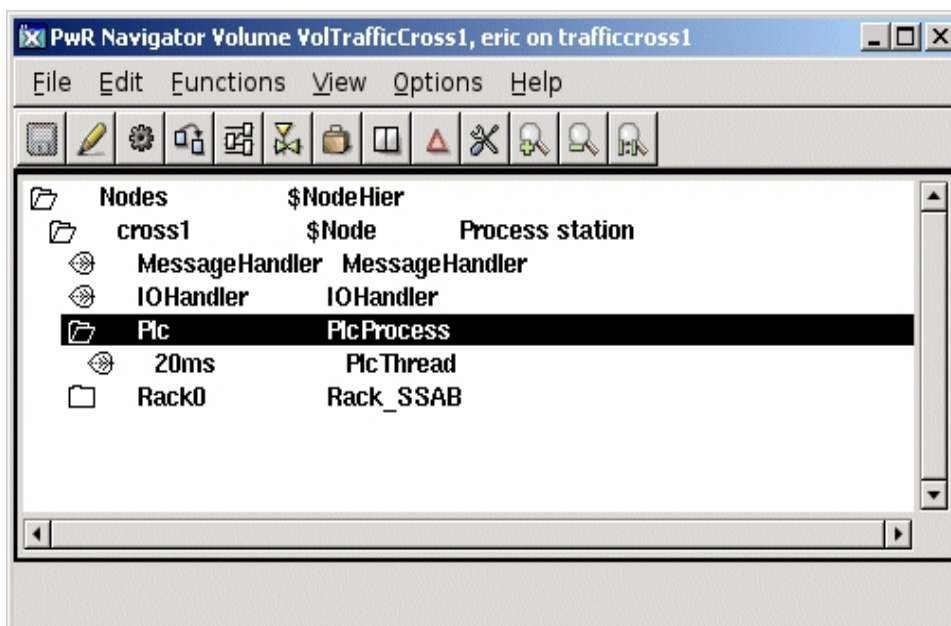
Fig Timebase configuration of the PLC program
